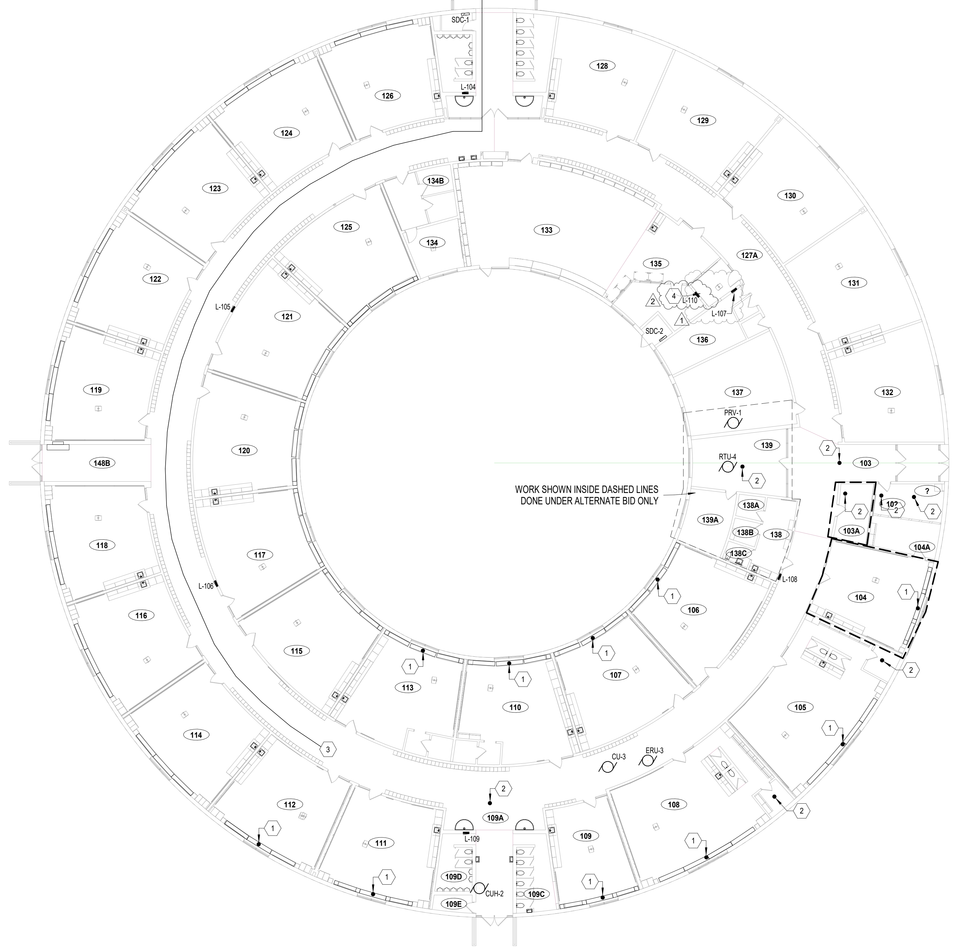
1 FIRST FLOOR MOTORS AND PANELBOARDS PLAN E6.1 1/16" = 1'-0" NORTH
