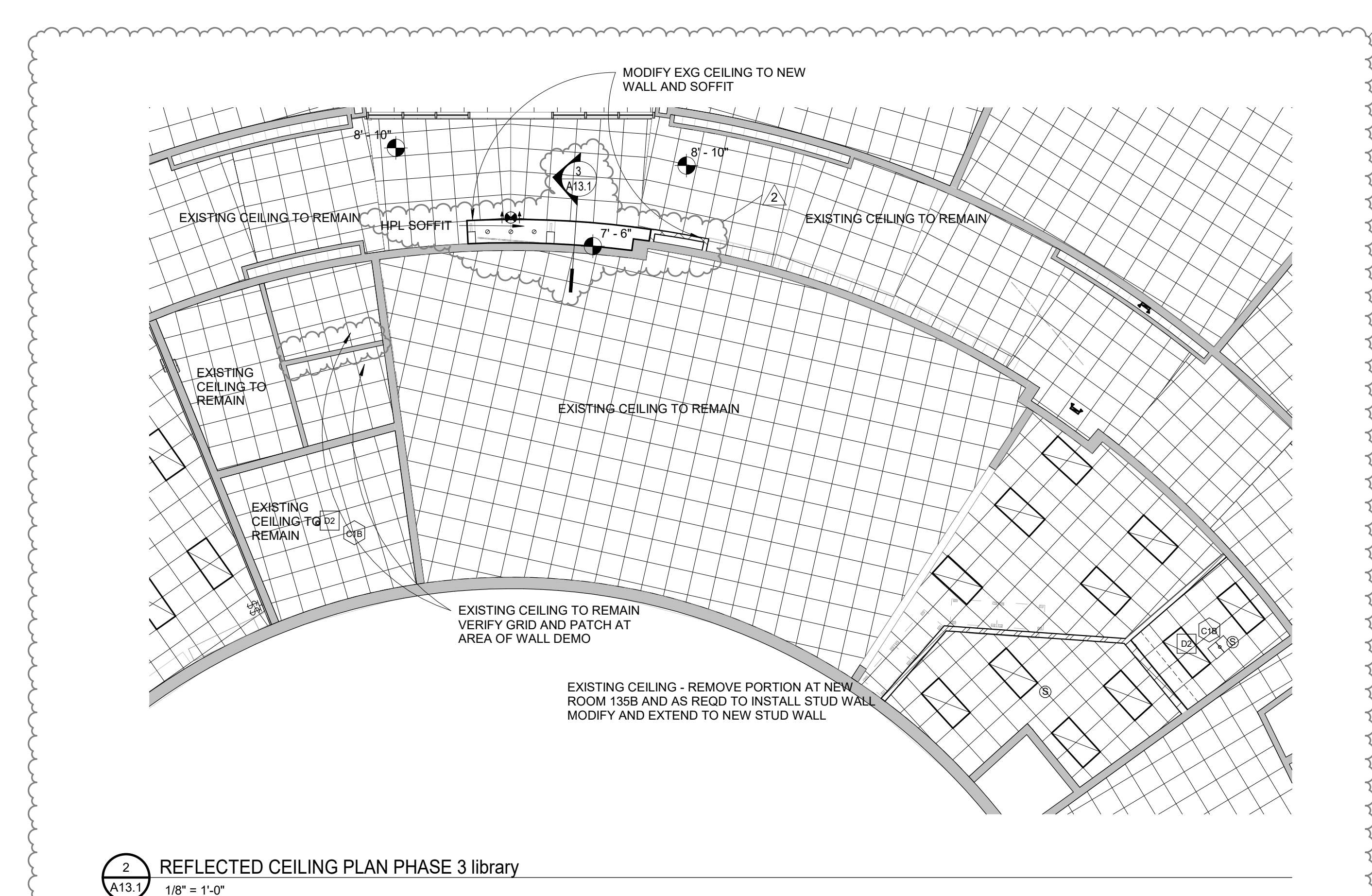
1 REFLECTED CEILING PLAN PHASE 3 1/8" = 1'-0"
